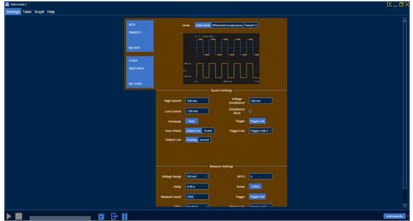
Use the Delta Mode App to apply an alternating source current to a DUT to derive a Delta voltage and low resistance measurement.
