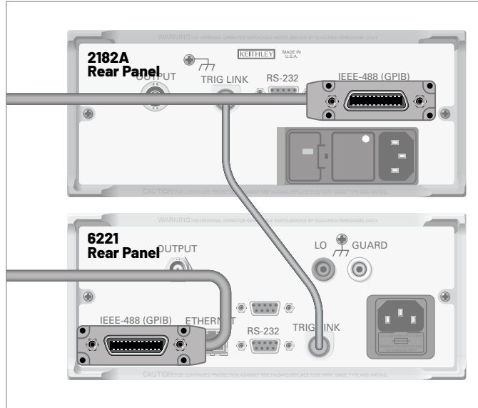
Connect communication cables for Delta Mode App as shown.
